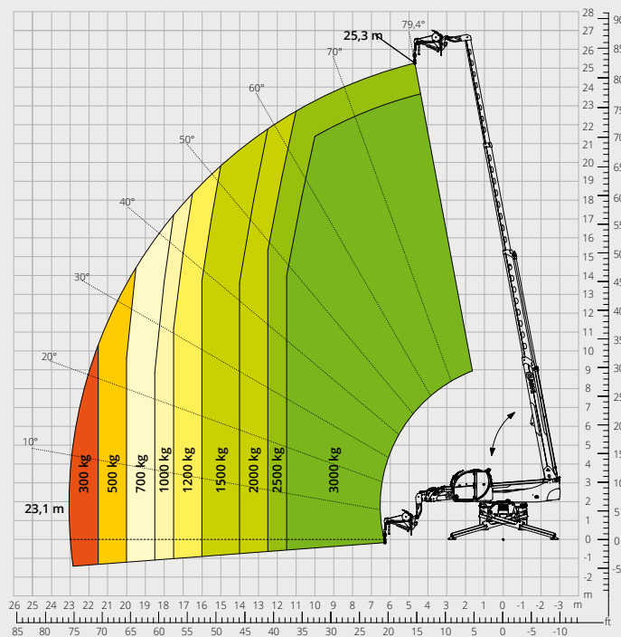
Load chart with JIB WITH WINCH, 3,000 kg ATT - 04 - 019
