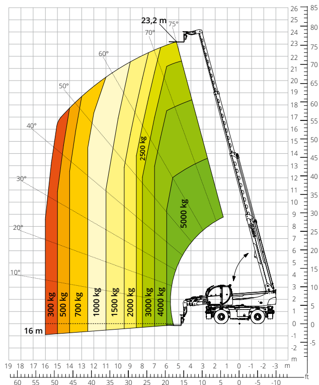
Load chart FRONT ATTACHMENT ON TYRES ATT-03-004
