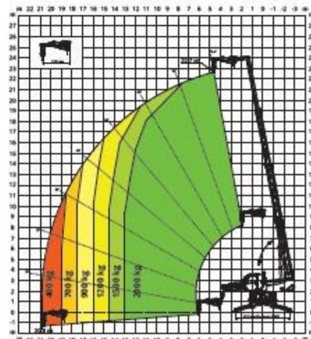
JIB WITH WINCH 2,000 kg
