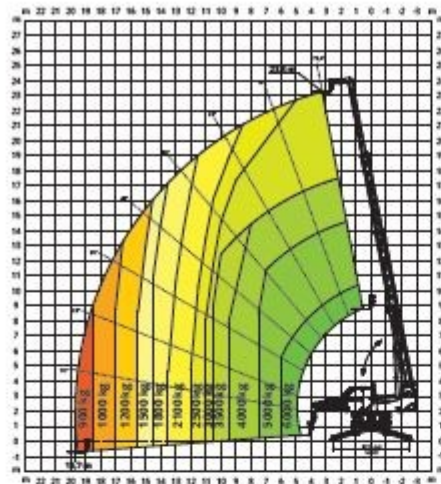
WINCH 3,500 kg
