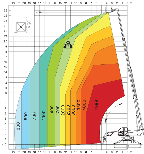
360° fully extended stabilizers load chart with forks
