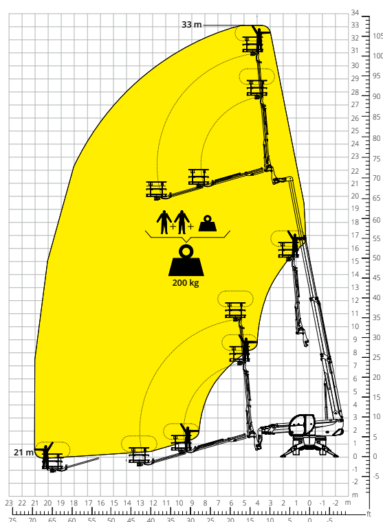
Load chart with TELESCOPIC PLATFORM 200 kg - 10 m ATT - 01 - 022
