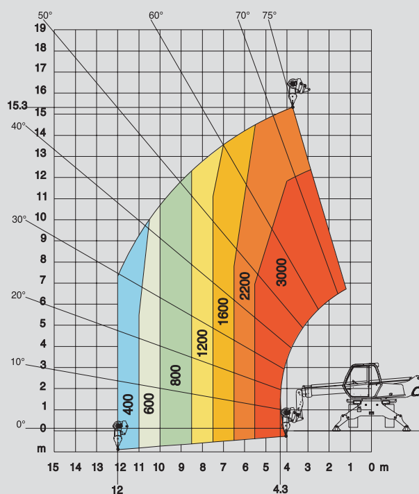
ROTATION ON STABILISERS WITH 3T WINCH
