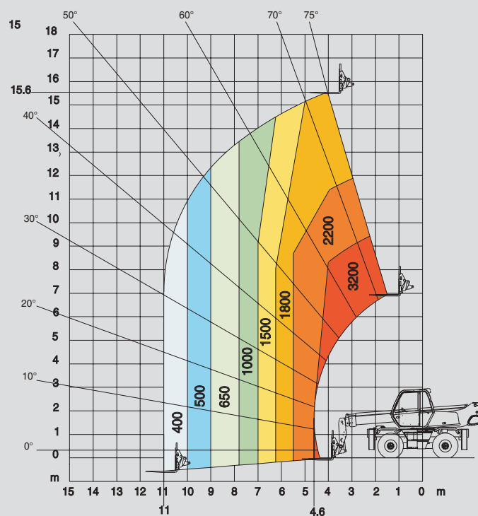
ROTATION ON STABILISERS WITH 3T WINCH
